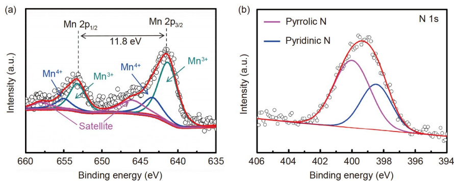
Figure 2 (Color online) XPS fitting results of Mn 2p_{1/2} and Mn 2p_{3/2} (a) and N 1s (b) of \text{MnO}_2@C-0.3 material.
