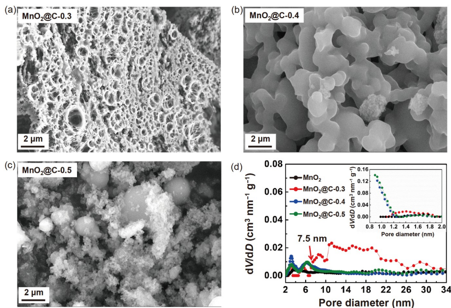
Figure 4 (Color online) (a)–(c) SEM morphologies of \text{MnO}_2@\text{C} materials; (d) pore size distribution curves of \text{MnO}_2 and \text{MnO}_2@\text{C} materials.
